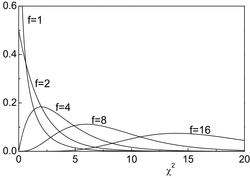
Fig. 3.20. \chi^2 distribution for different degrees of freedom.
