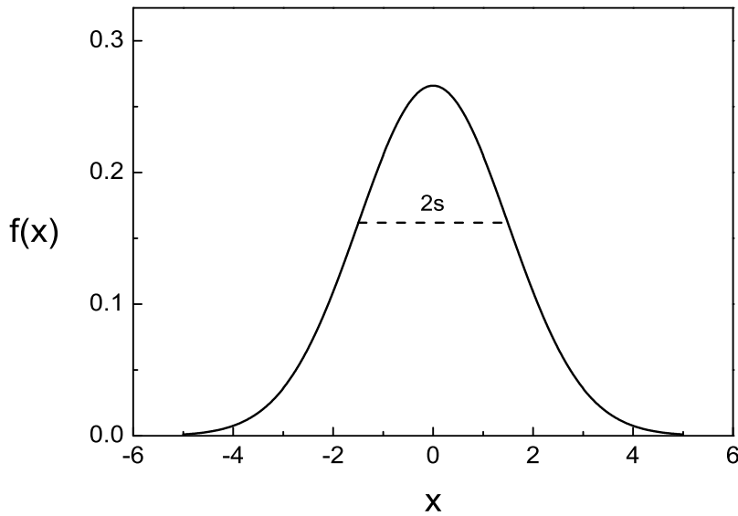
Fig. 3.5. Normal distribution.
